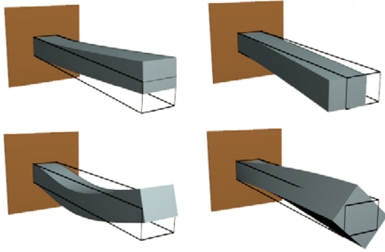
Figure 15: The first four dominant low frequency mode shapes \Phi_1, \dots, \Phi_4 of a constrained bar. The distortion inherent to linear modal analysis is most evident in the bottom right figure [BJ05].
